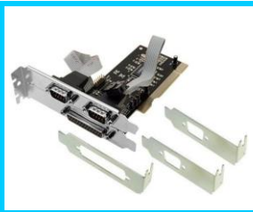
PCI-09(LP) PCI To ComPort+Parallel w/ Low-Profile ask
