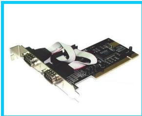
PCI-07 PCI To ComPort Card ASK
